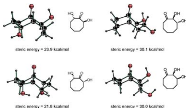
Figure 2. Global minimum energy conformations of the 2,3- and 2,8-dihydroxycyclooctanones.
