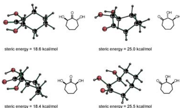
Figure 1. Global minimum energy conformations of the 2,3- and 2,7-dihydroxycycloheptanones.
